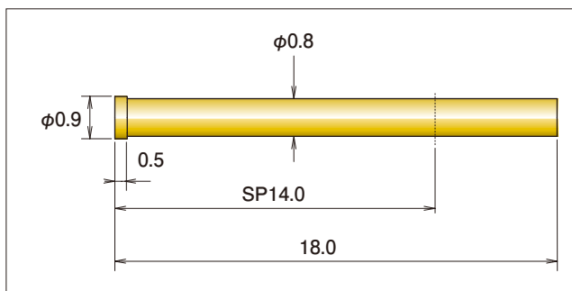
K2-0.58S-1-18L-SP14-2 (S058-140-03)
