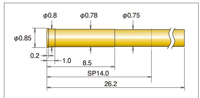
K2-0.58S-3-26.2L-SP14-2 (S058-140-04)
