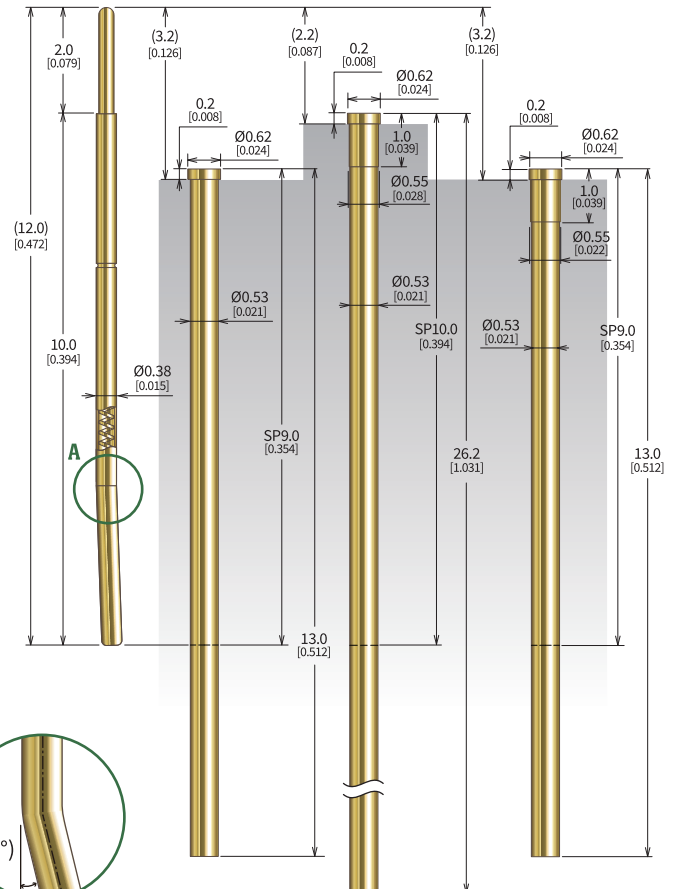
抜け止め用曲げ加工付 Bending for retention
